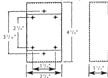
Surface Mounting: DHBB (backbox)
